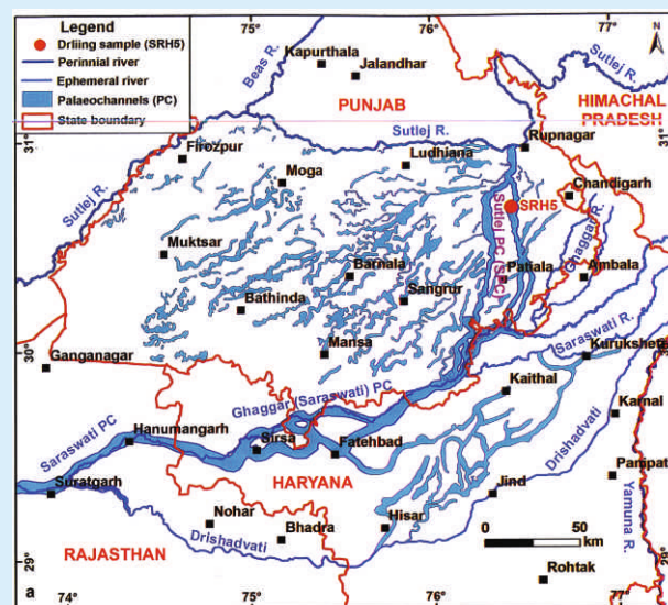
Fig.2: Linkages of Sutlej palaeochannels with Ghaggar (Sarasvati) palaeochannels in northwest India. Location of drill hole sample (SRH5) on SPC used for dating.
