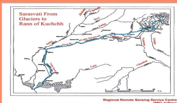
Sarasvati from Glaciers to Rann of Kutch
