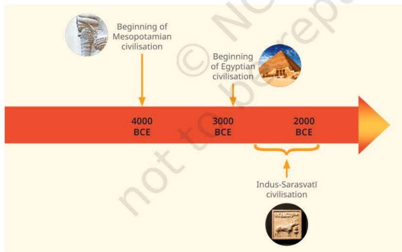
Fig. 6.2. Timeline showing the period of the Indus-Sarasvatī civilisation, from about 2600 to 1900 BCE.
